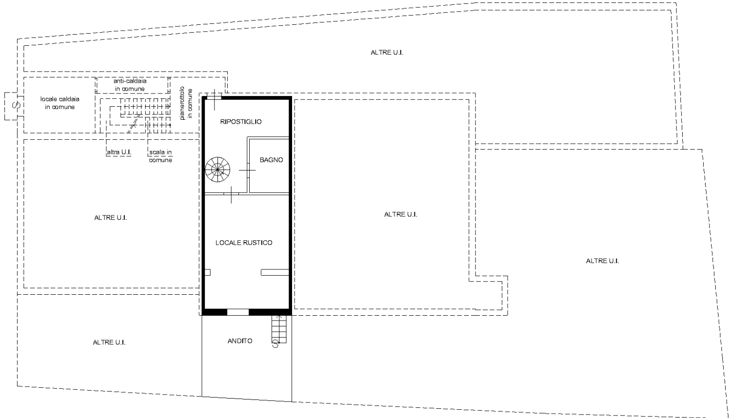
PIANO INTERRATO (-1) H=2.30 m
