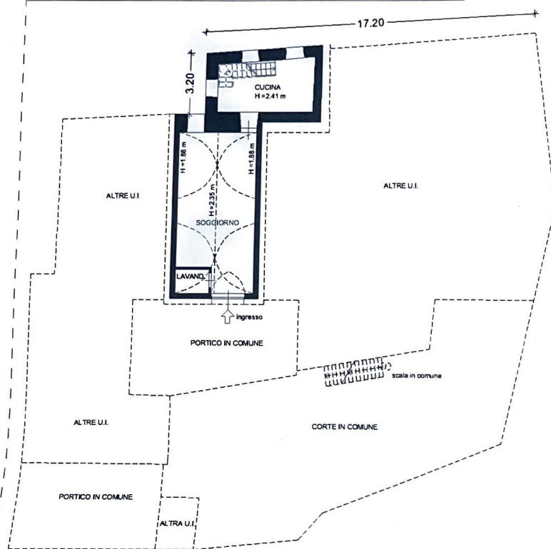
PIANO TERRA (PT) H max = 2.35 m H min = 1.88 m
