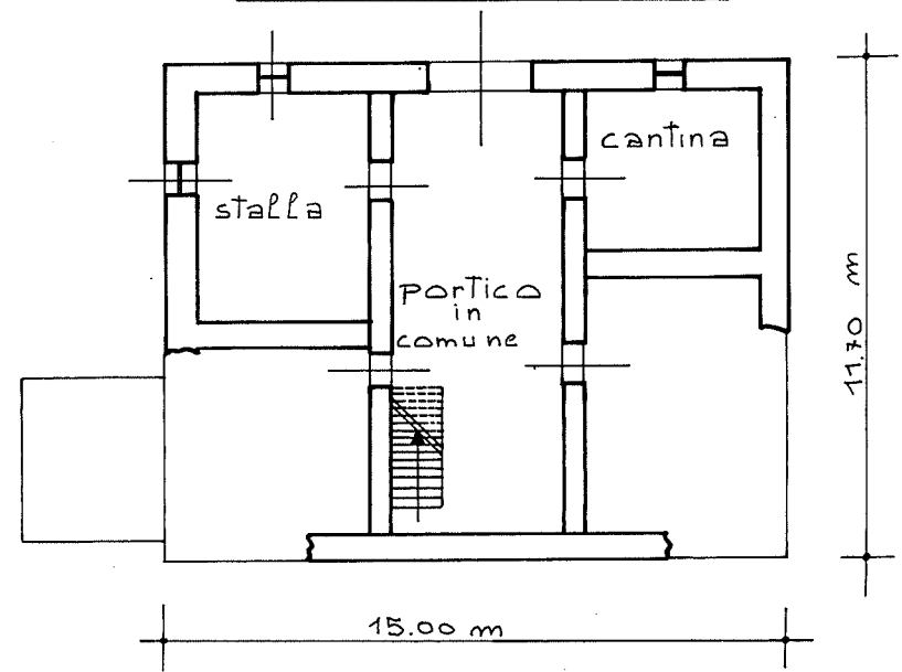
PIANO TERRA (PT) H=300
